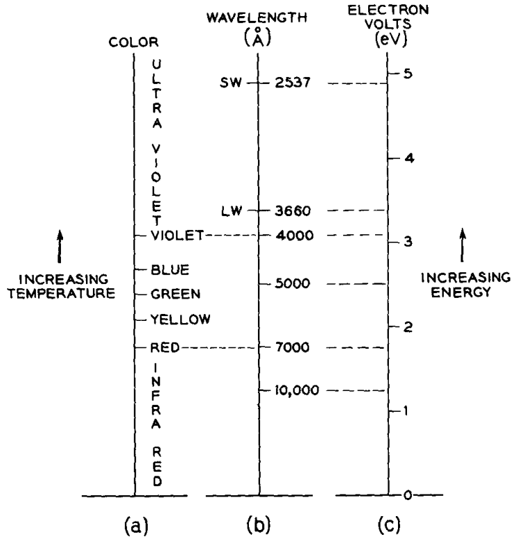
Fig. 1. Colors, wavelengths (Å), and energy (eV) For spectral pure light (SW is short and LW long wavelength ultraviolet).
