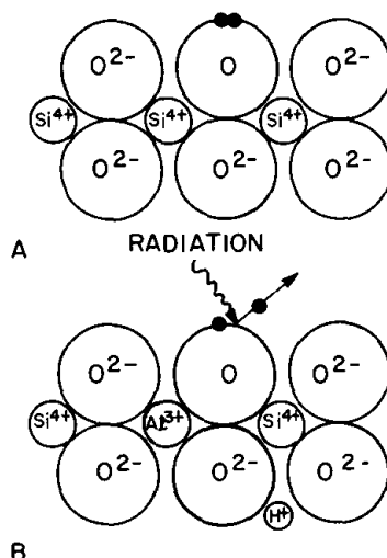
Fig. 4. Quartz structure (schematic): (A) normal, (B) containing Al 3+ substituted for Si 4+ with an H + for charge neutrality. Radiation ejects one of a pair of electrons from an O 2- and leaves a "hole" color center of smoky quartz.
