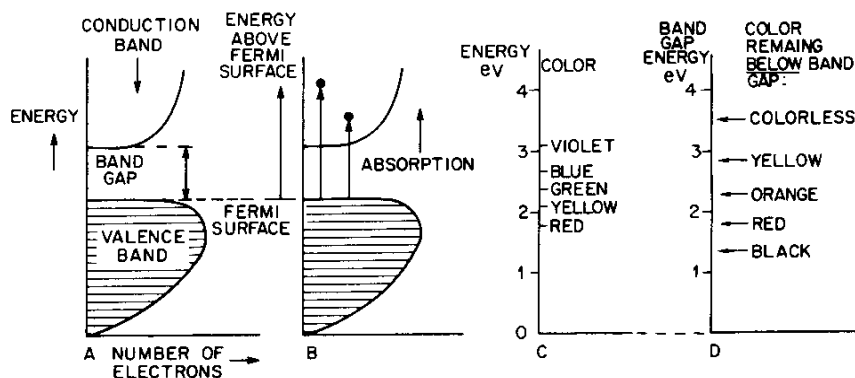
Fig. 7. Band diagrams of a typical semiconductor (A), showing light absorption transmissions (B); the dependence of color on the energy of light in (C) leads to the color remaining for various band gap energies in (D).
